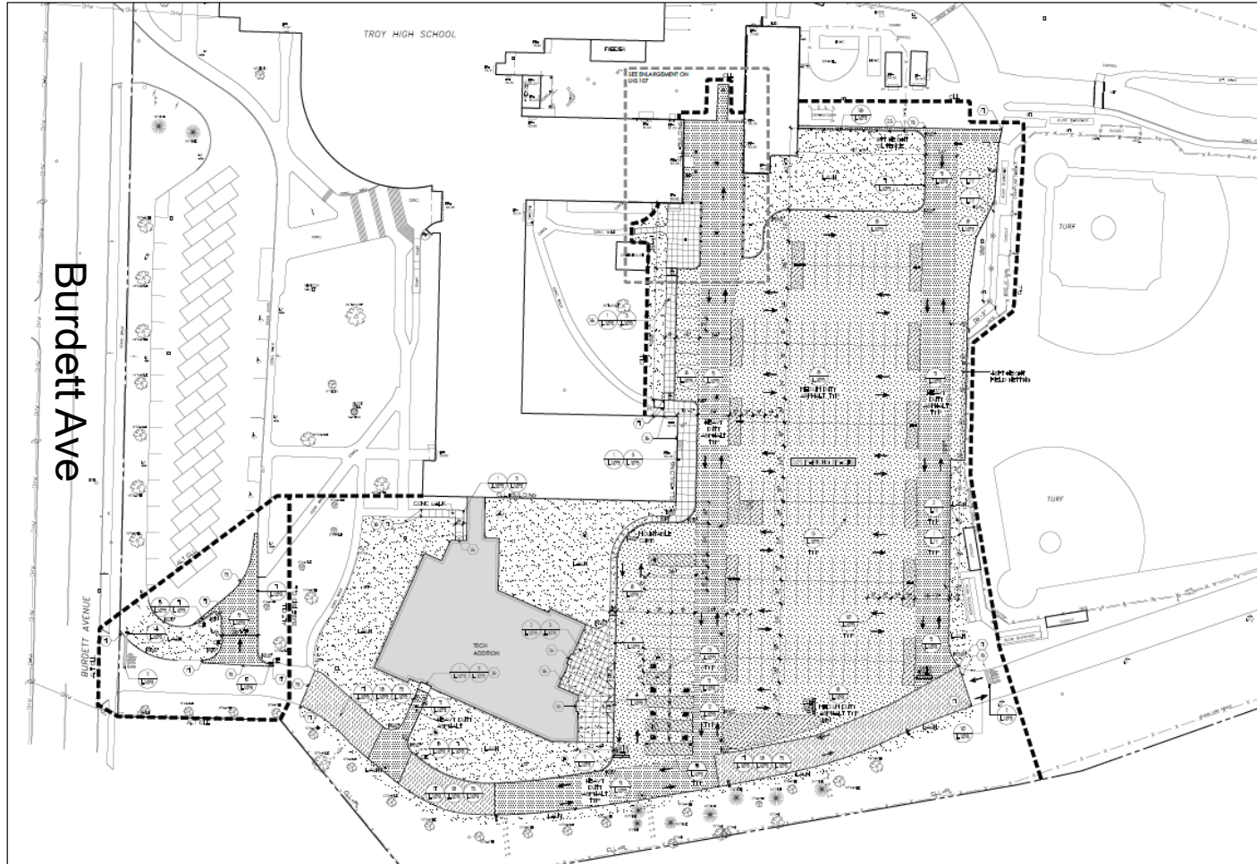
SITE LAYOUT PLAN - TROY HIGH SCHOOL
